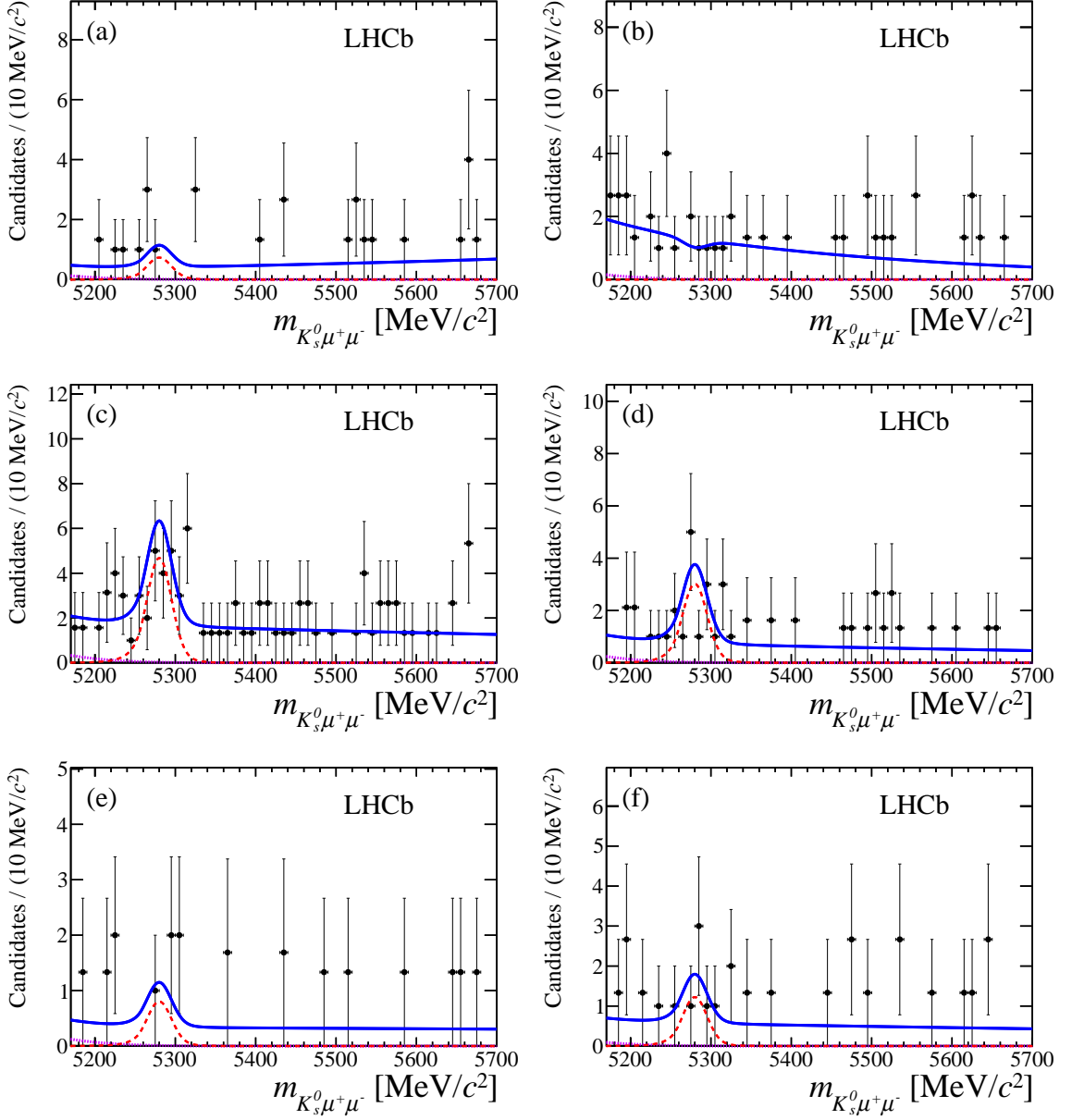
Figure 2: Mass distributions and fits for B^0 \rightarrow K_s^0 \mu^+ \mu^- decays in the individual q^2 bins for the D category. The figures are ordered as in Table 2 of the main paper.
