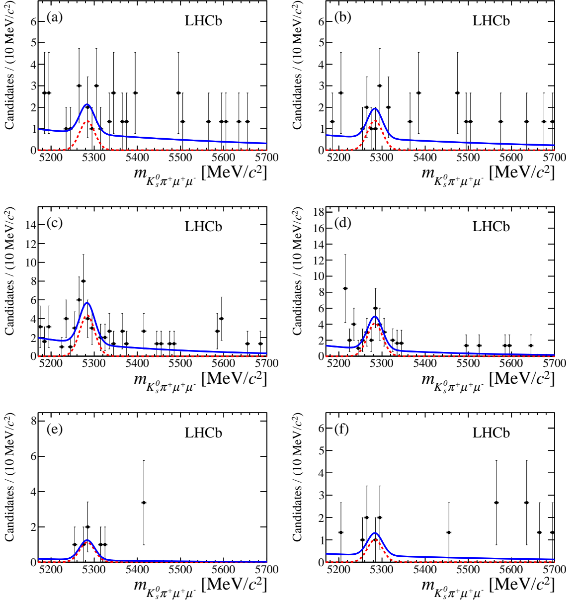
Figure 4: Mass distributions and fits for B^+ \rightarrow K^{*+} \mu^+ \mu^- decays in the individual q^2 bins for the D category. The figures are ordered as in Table 3 of the main paper.
