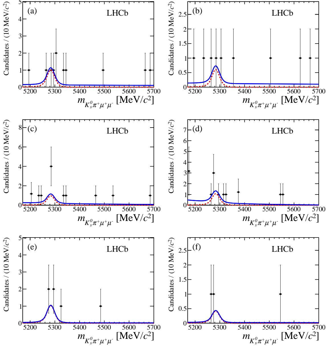
Figure 3: Mass distributions and fits for B^+ \rightarrow K^{*+} \mu^+ \mu^- decays in the individual q^2 bins for the L category. The figures are ordered as in Table 3 of the main paper.
