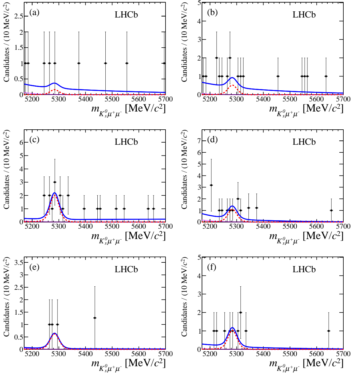
Figure 1: Mass distributions and fits for B^0 \rightarrow K_s^0 \mu^+ \mu^- decays in the individual q^2 bins for the L category. The figures are ordered as in Table 2 of the main paper.
