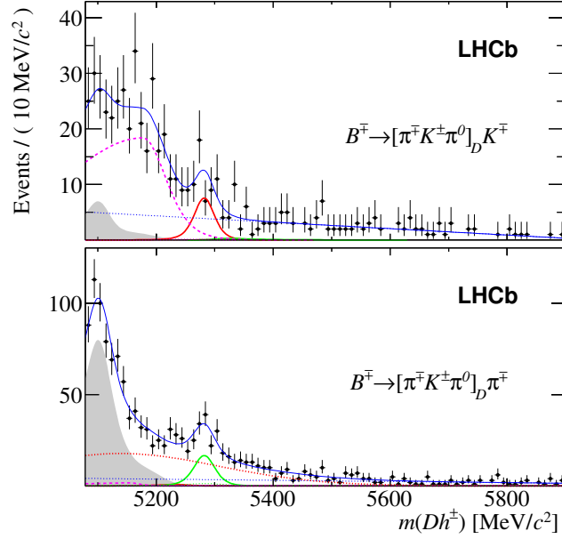
Figure S.1: Charge-integrated invariant mass distributions of candidates shown in Fig. 2 passing the B^{\mp} \rightarrow [\pi^{\mp} K^{\pm} \pi^0]_D h^{\mp} selection.
