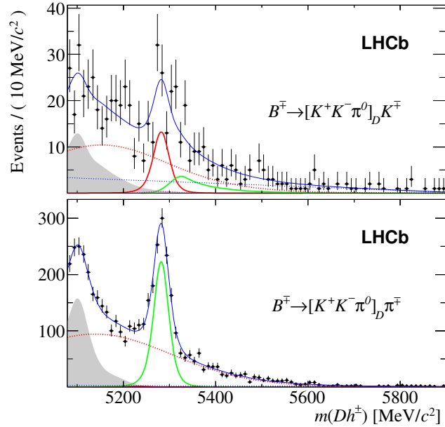
Figure S.2: Charge-integrated invariant mass distributions of candidates shown in Fig. 4 passing the B^{\mp} \rightarrow [K^+ K^- \pi^0]_D h^{\mp} selection.
