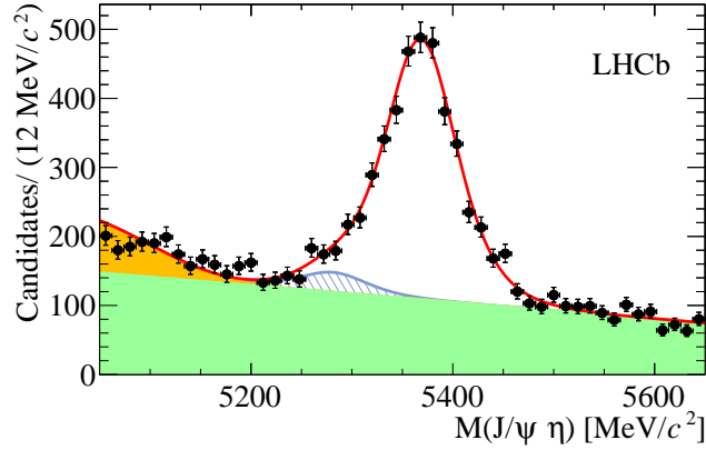
Figure 1: Mass distribution for the combined 2011 and 2012 dataset. The fit model described in the text is superimposed (red line). The sum of the partially reconstructed and combinatorial background is shown (solid yellow) and the B^0 component (open blue).
