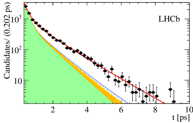
Figure 2: Time distribution for the combined 2011 and 2012 dataset. The fit model described in the text is superimposed (red line). The sum of the partially reconstructed and combinatorial background is shown (solid yellow) and the B^0 component (open blue).
