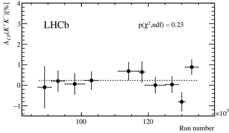
Figure 4: A_{CP}(K^- K^+) as a function of the run number of the LHC. The full analysis is performed for each of the sub-samples individually. Additionally, the p -value for the hypothesis of independency is given.
