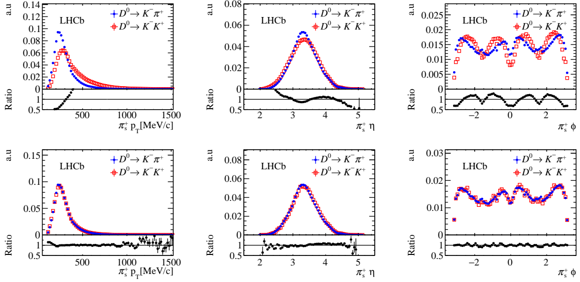
Figure 3: Normalised kinematic distributions of the \pi_s^+ in the weighting of D^0 \rightarrow K^- K^+ candidates to D^0 \rightarrow K^- \pi^+ candidates. In the top row, they are shown before, and in the bottom row, after weighting. The data sample taken in 2012 with magnet polarity up is shown.
